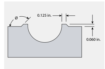
Figure 7: A rib is added to the tool design. The rib follows the contours of the mold cavity.
