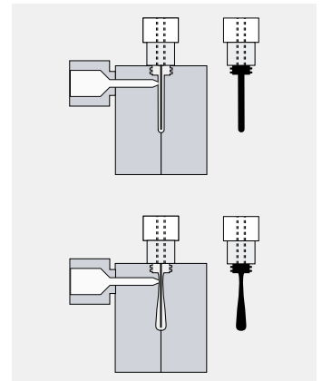
Figure 5: Varying the shape of the preform offers variable wall thickness.
