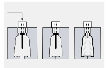
Figure 6: After the preform is molded, it is transferred to the blow mold tool and inflated.
