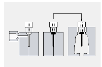
Figure 4: Preform is injection molded and transferred to the blow molding tool.
